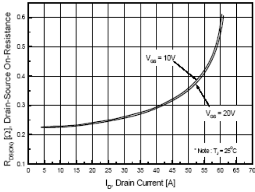
Figure 3. On-Resistance Variation
