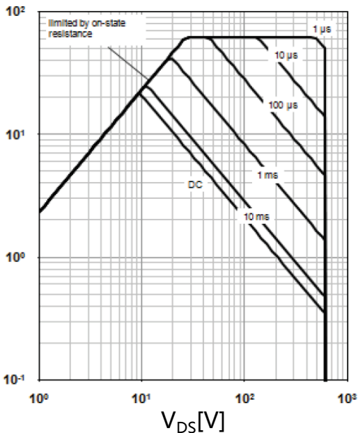
Safe operating area T_C=25^\circ\text{C}
