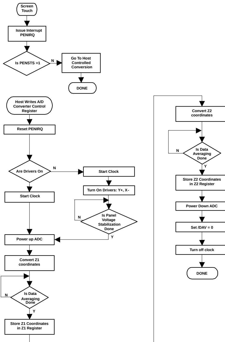
Figure 52. Z Coordinate Reading Initiated by Host
