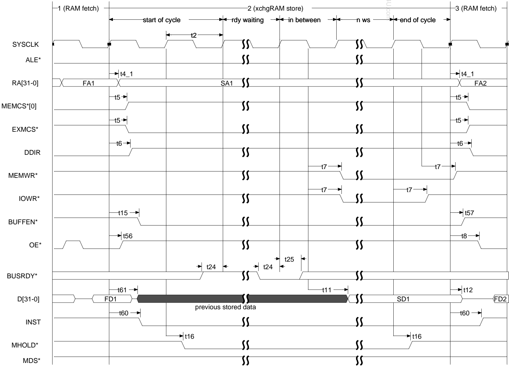
Figure 14. EXCHANGE RAM Store with BUSRDY* and n Waitstates
