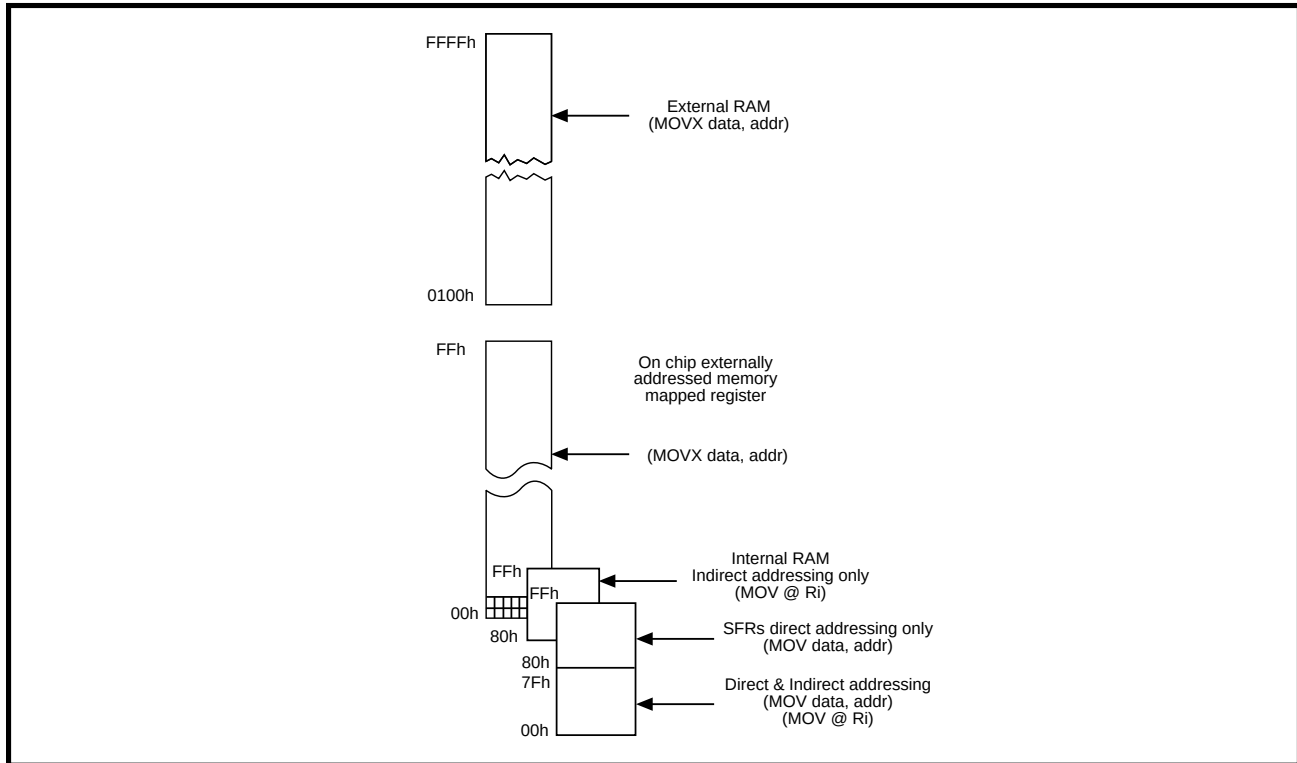
FIGURE 6: Memory Map
