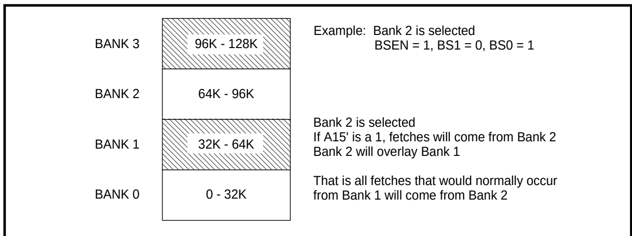
FIGURE 1: Bank Select
