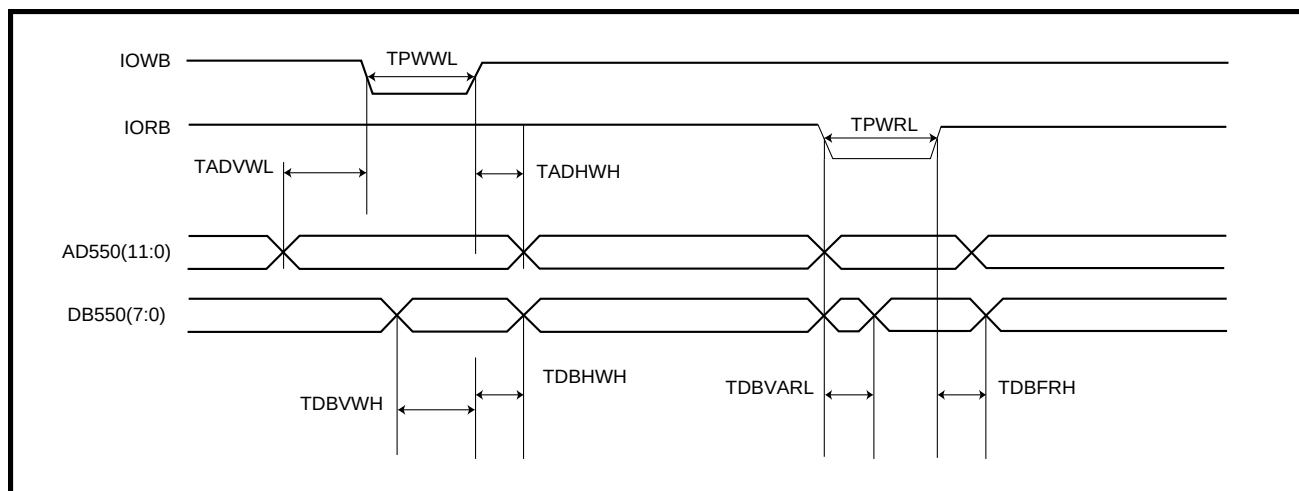
FIGURE 10: AC Timing
