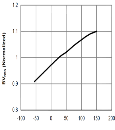
Figure 5: Break Down vs. Junction Temperature
