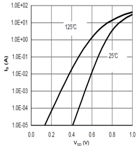
Figure 6: Body-Diode Characteristics
