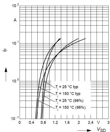
Figure 6: Body-Diode Characteristics
