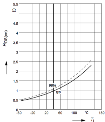
Figure 4: On-Resistance vs. Junction Temperature
