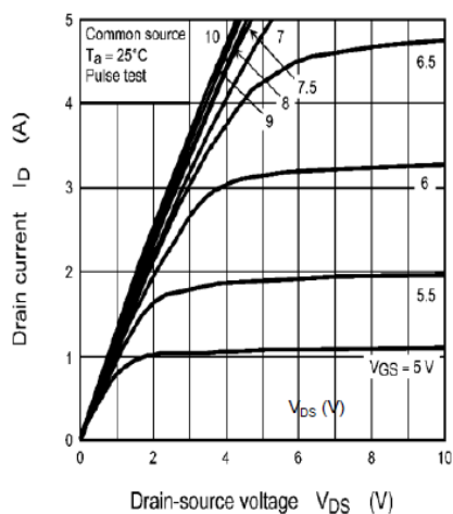
Figure 1: On-Region Characteristics@25°C
