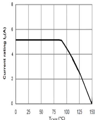
Figure 12: Current De-rating
