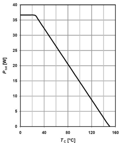
Figure 3: Power Dissipation
