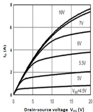
Figure 2: On-Region Characteristics@125°C
