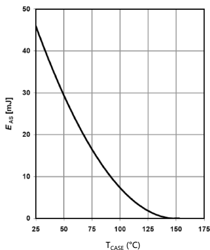
Figure 11: Avalanche energy
