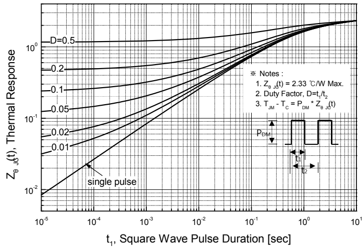
Figure 11-2. Transient Thermal Response Curve for TSF12N60M
