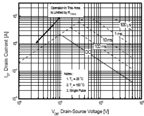
Figure 9-2. Maximum Safe Operating Area for TSF2N60MZ
