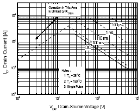
Figure 9-1. Maximum Safe Operating Area for TSP2N60MZ
