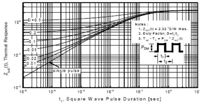
Figure 11-1. Transient Thermal Response Curve for TSP2N60MZ
