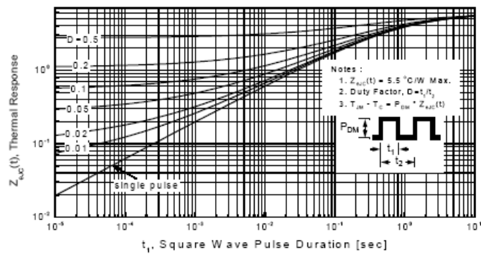
Figure 11-2. Transient Thermal Response Curve for TSF2N60MZ
