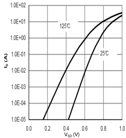
Figure 6: Body-Diode Characteristics
