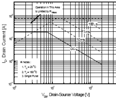
Figure 9-1. Maximum Safe Operating Area for TSP640M
