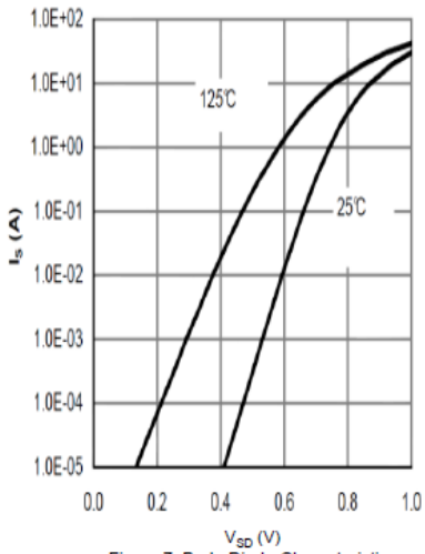
Figure 7: Body-Diode Characteristics
