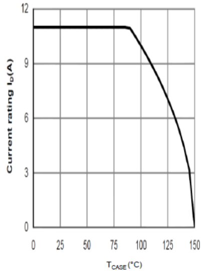
Figure 15: Current De-rating
