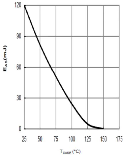
Figure 14: Avalanche energy
