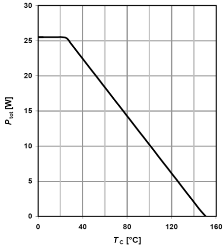
Figure 3: Power Dissipation
