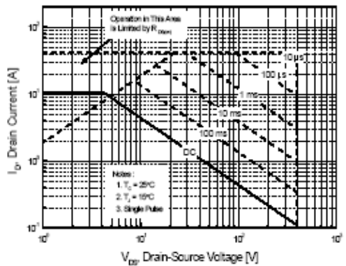
Figure 9-2. Maximum Safe Operating Area for TSF740M
