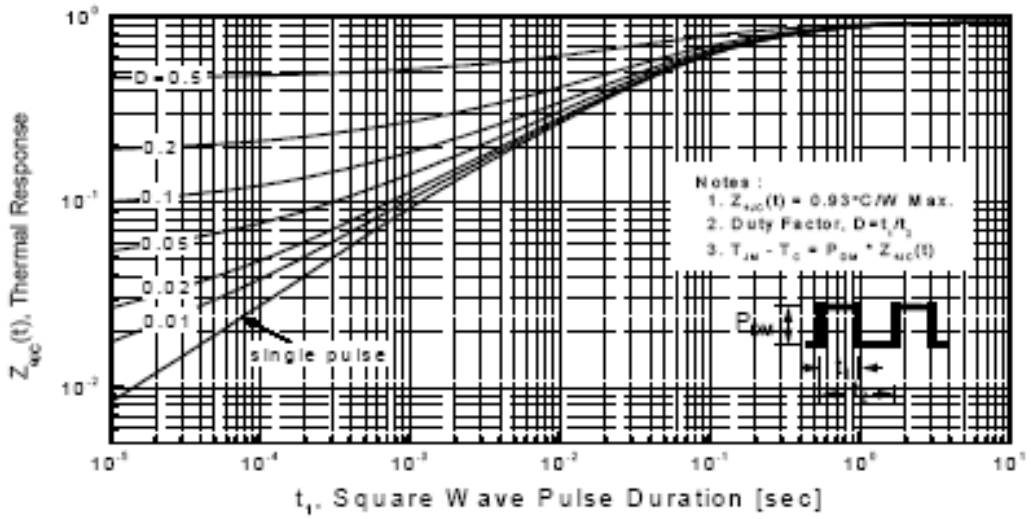
Figure 11-1. Transient Thermal Response Curve for TSP740M
