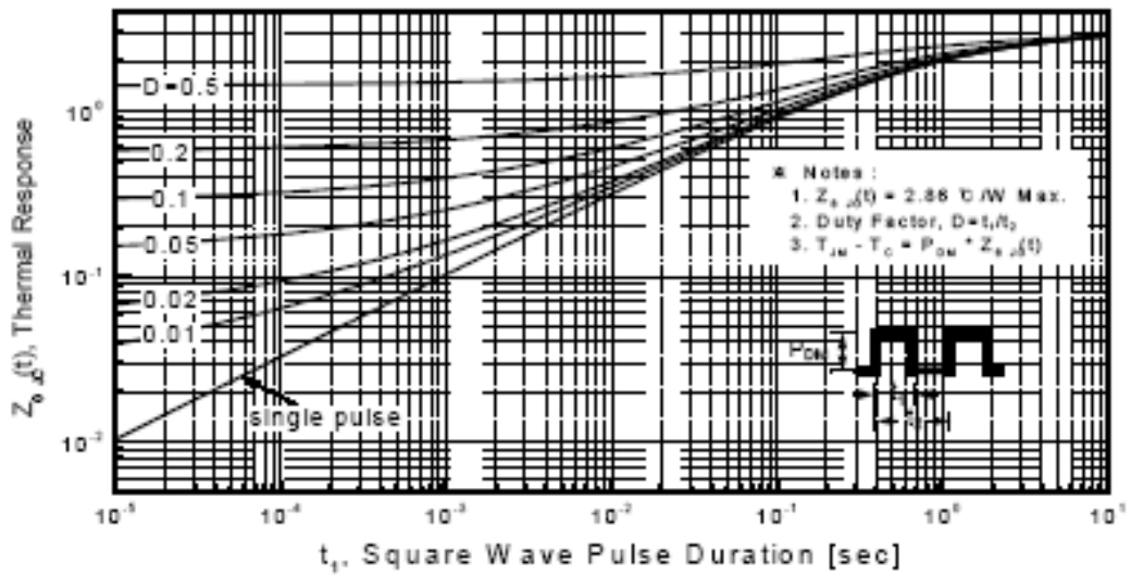
Figure 11-2. Transient Thermal Response Curve for TSF740M
