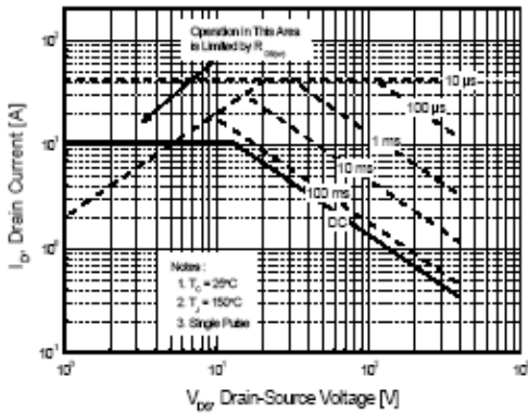
Figure 9-1. Maximum Safe Operating Area for TSP740M
