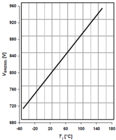
Figure 11: Break Down vs. Junction Temperature
