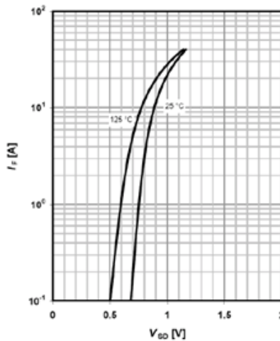
Figure 6: Body-Diode Characteristics
