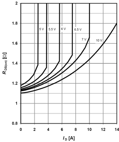
Figure 6: On-Resistance vs. Drain Current, T J =125°C
