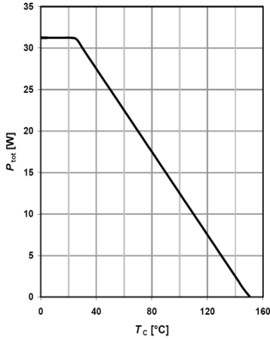
Figure 4 : Power dissipation
