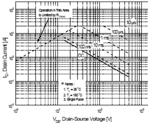
Figure 9-1. Maximum Safe Operating Area for TSP830M
