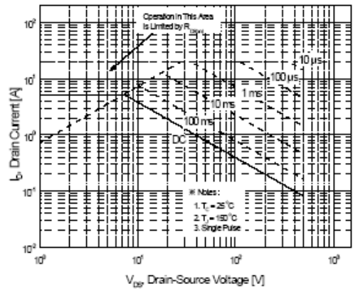
Figure 9-2. Maximum Safe Operating Area for TSF830M
