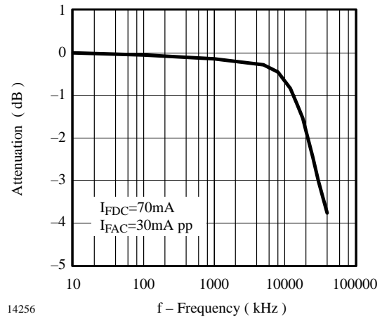
Figure 11. Attenuation vs. Frequency
