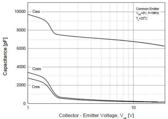
Capacitance characteristics
