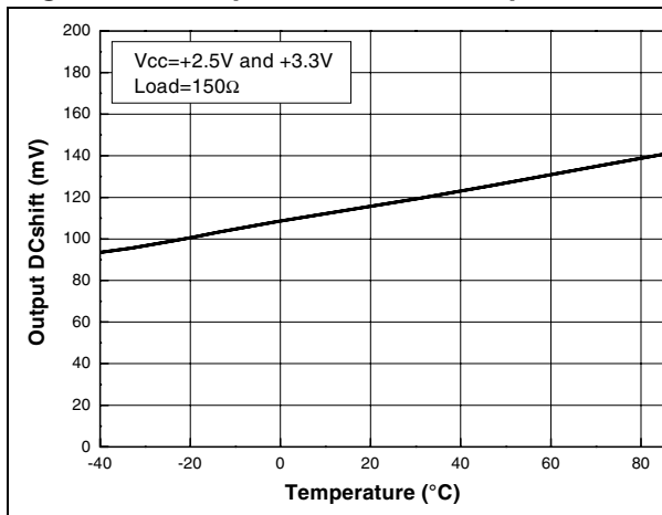
Figure 21. Output DC shift vs. temperature
