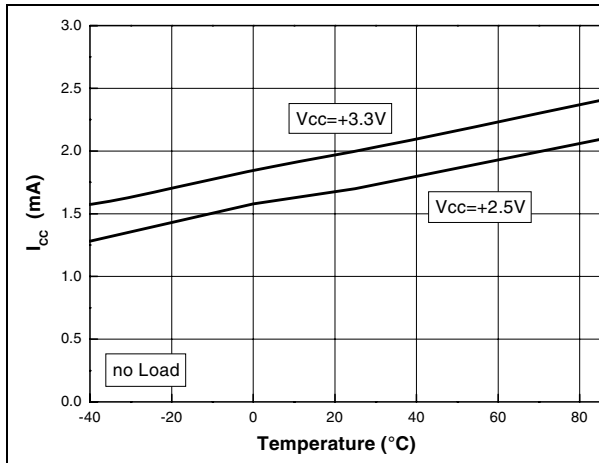
Figure 19. I cc vs. temperature
