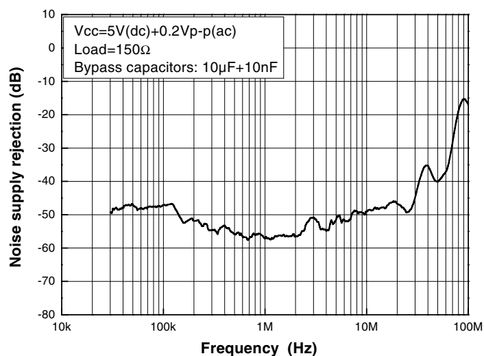
Figure 24. Supply noise rejection
