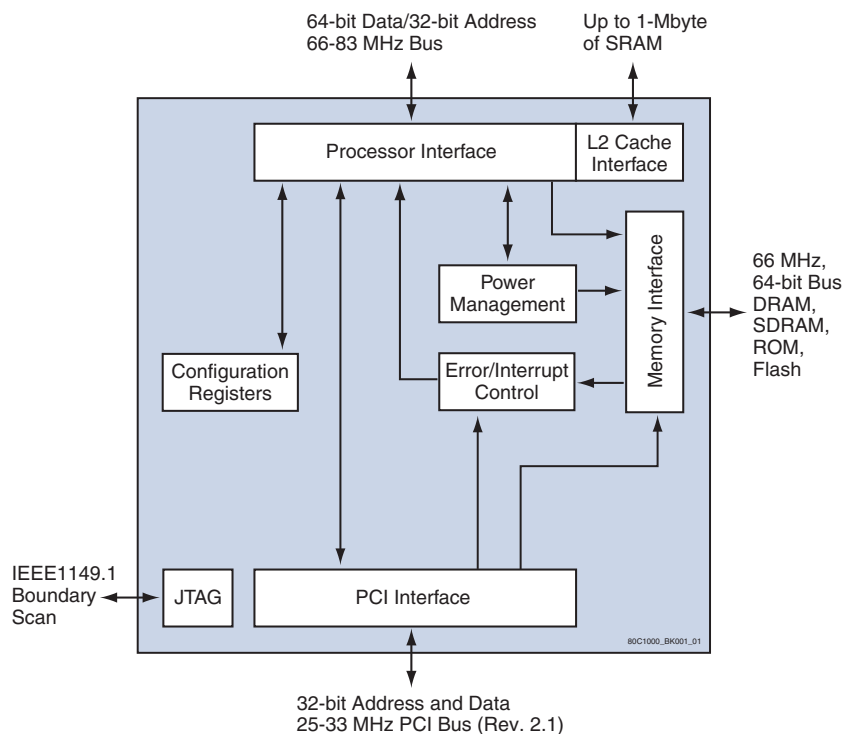
Figure 1: Tsi106 Block Diagram
