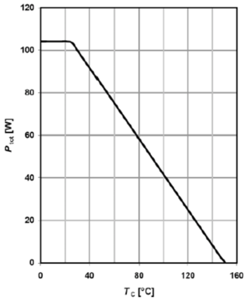
Power dissipation
