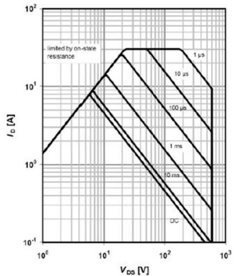
Safe operating area T_c=80^\circ\text{C}
