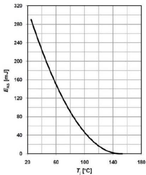
Avalanche energy
