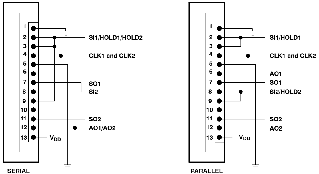
Figure 9. Operational Connections
