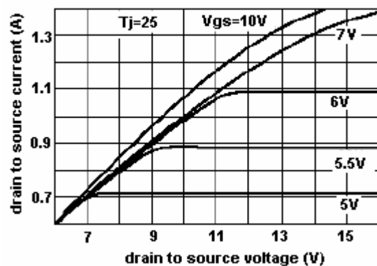
Output Characteristic
