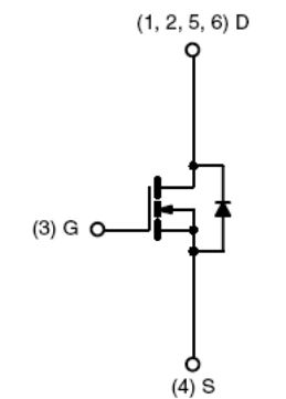
N-Channel MOSFET
