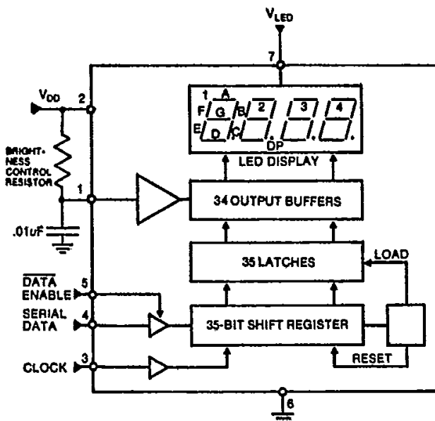
FIGURE 1—Block Diagram
