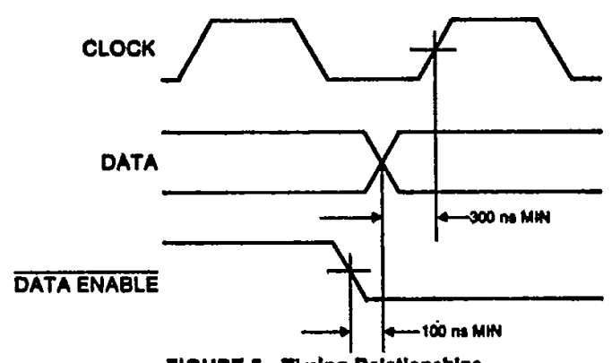
FIGURE 5—Timing Relationships
