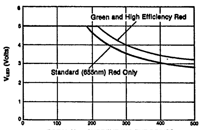
TOTAL V_{LED} CURRENT INC EXT DRIVES FIGURE 2—Max V_{LED} vs I_{LED} Circuit Per Figure 1
