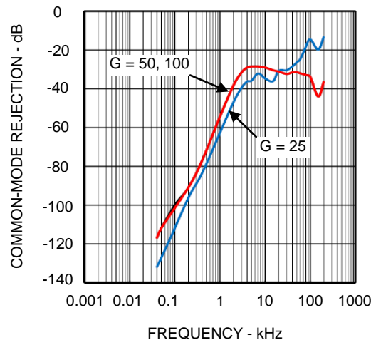
Common-Mode Rejection vs Frequency
