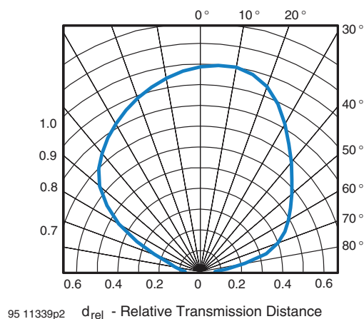
Fig. 12 - Vertical Directivity
