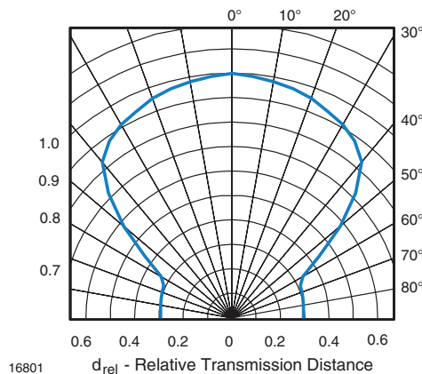
Fig. 11 - Directivity
