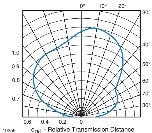
Fig. 12 - Vertical Directivity
