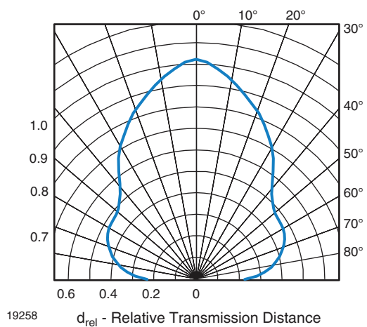
Fig. 11 - Horizontal Directivity
