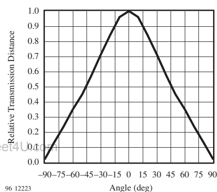
Figure 11. Directivity
