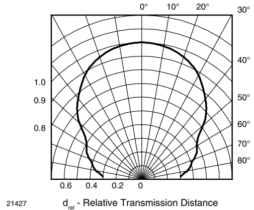
Fig. 11 - Horizontal Directivity
