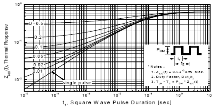
Figure 11-1. Transient Thermal Response Curve for TSP16N50M
