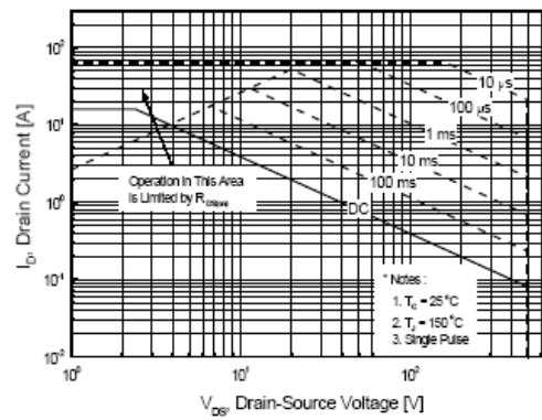
Figure 9-2. Maximum Safe Operating Area for TSF16N50M
