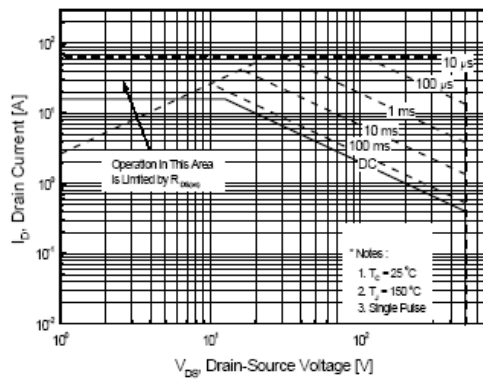
Figure 9-1. Maximum Safe Operating Area for TSP16N50M
