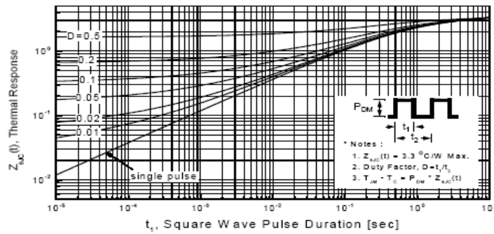
Figure 11-2. Transient Thermal Response Curve for TSF16N50M
