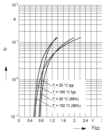
Figure 6: Body-Diode Characteristics
