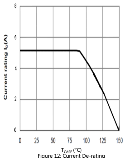
Figure 12: Current De-rating
