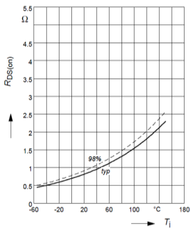
Figure 4: On-Resistance vs. Junction Temperature
