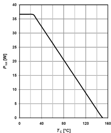
Figure 3: Power Dissipation
