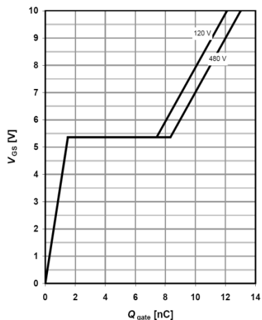
Figure 7: Gate-Charge Characteristics
