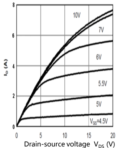
Figure 2: On-Region Characteristics@125°C
