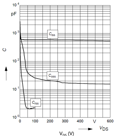
Figure 8: Capacitance Characteristics
