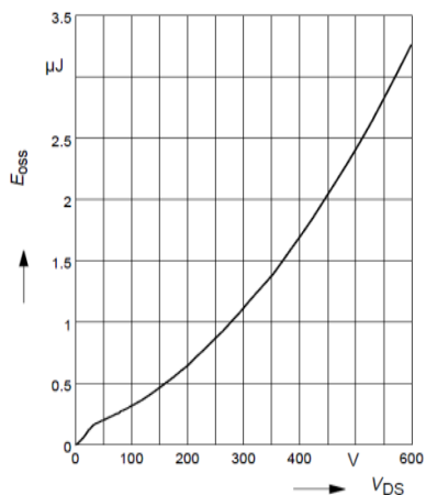
Figure 9: C_{oss} stored Energy
