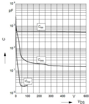
Figure 8: Capacitance Characteristics
