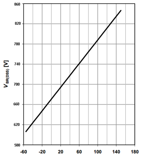
Drain-source breakdown voltage
