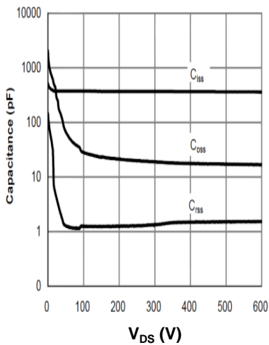
Figure 9: Capacitance Characteristics
