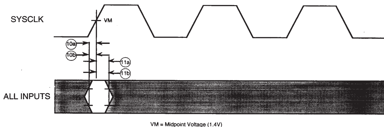
Figure 8 : Input timing diagram
