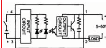
Connection Diagram
