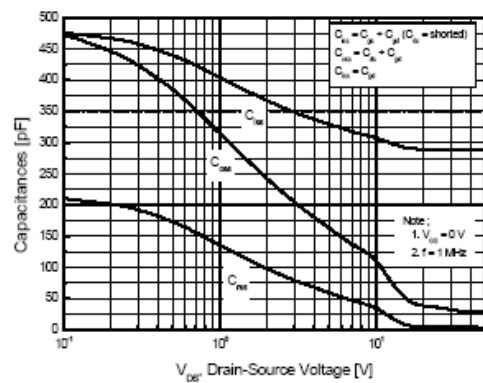
Figure 5. Capacitance Characteristics
