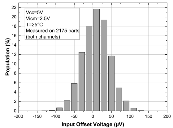
Figure 4. Input offset voltage distribution at V_{CC} = 5\text{ V} (TSV782)
