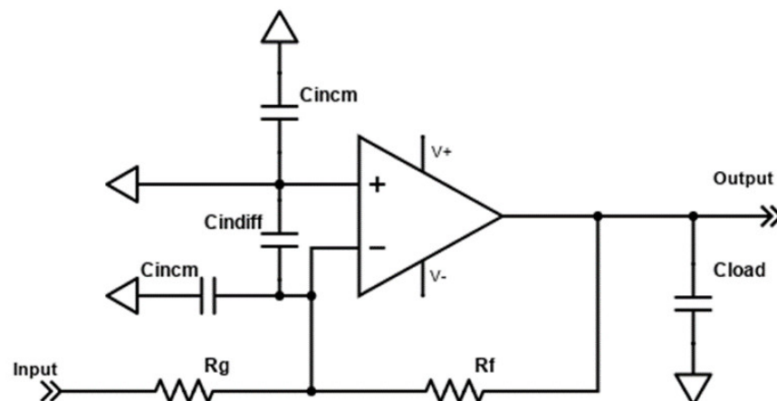
Figure 44. Inverting amplifier configuration with parasitic input capacitances
