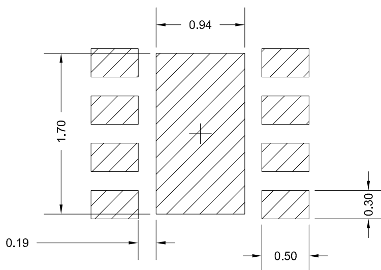
Figure 49. DFN8 2x2 recommended footprint
