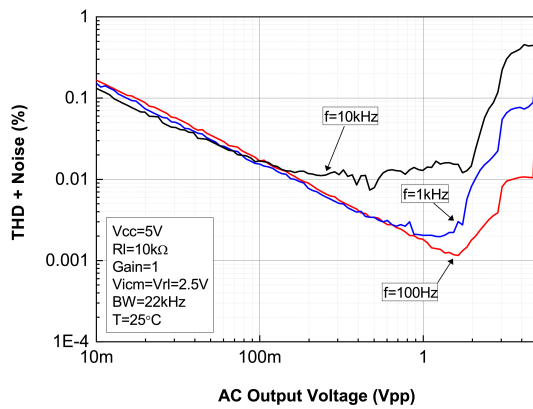
Figure 37. THD+N vs. output voltage
