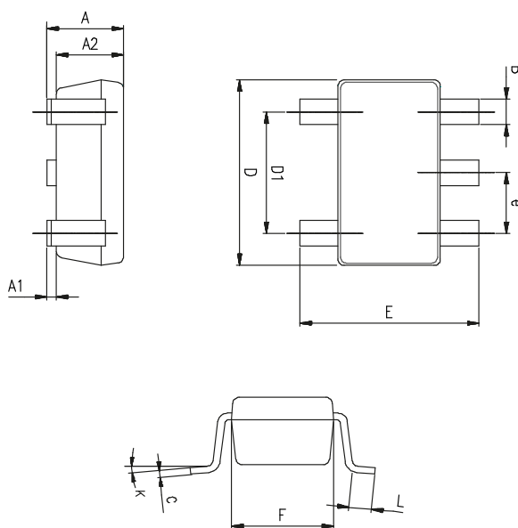
Figure 47. SOT23-5 package outline
