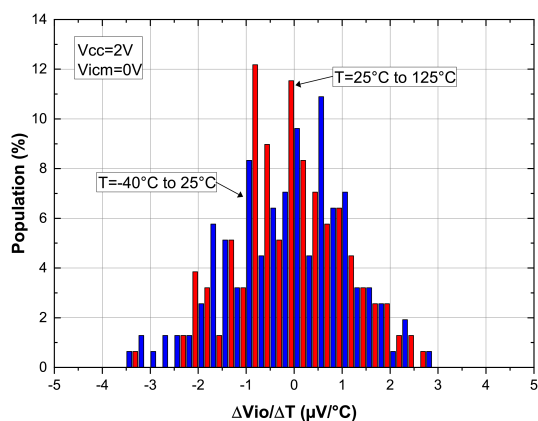
Figure 9. Input offset voltage thermal drift distribution at V_{CC} = 2\text{ V} (TSV782)
