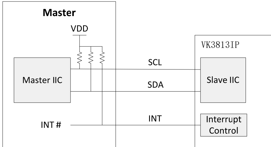
Figure6. IIC connect for master and VK3813IP
