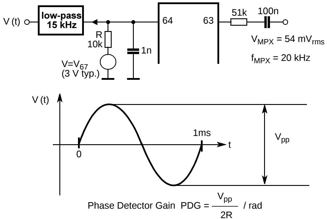
Figure 5-1 Definition of Phase Detector Gain
