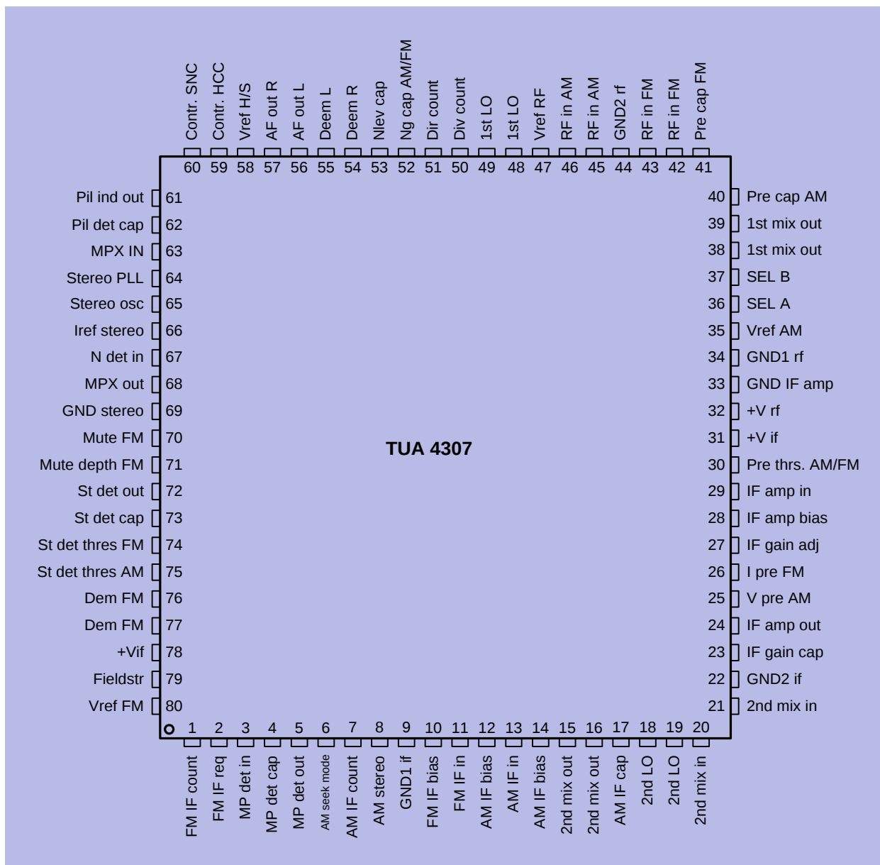
Figure 3-1 Pin Configuration
