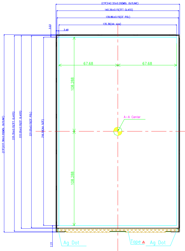
FRONT
