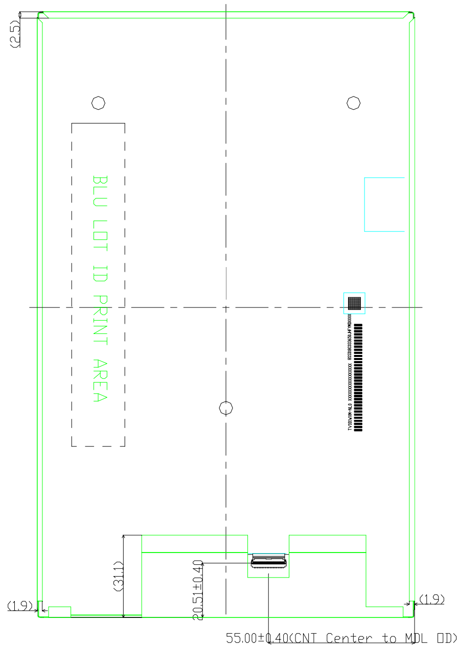
Figure 13. TFT-LCD Module Outline Dimensions (Rear view)
