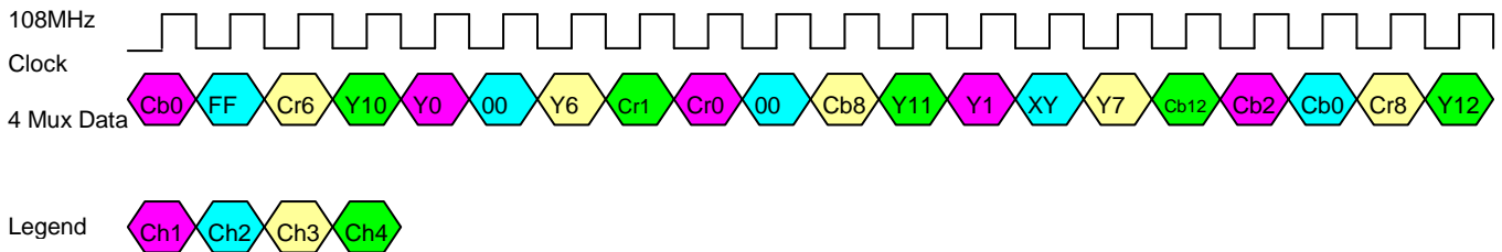
FIGURE 5. TIMING DIAGRAM OF 108MHZ 4 CH D1 TIME-DIVISION-MULTIPLEXED VIDEO DATA
