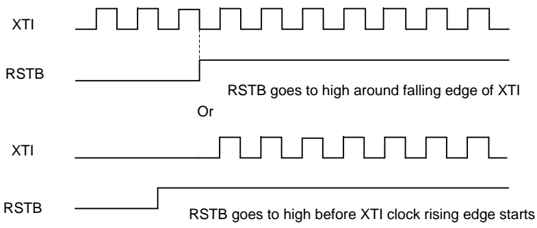
FIGURE 12. RSTB CONTROL FOR 108MHZ XTI INPUT
