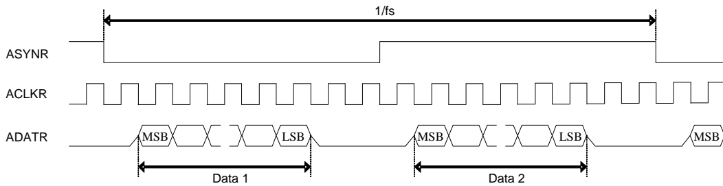
FIGURE 15. ACLKMASTER=0, RM_SYNC=0
