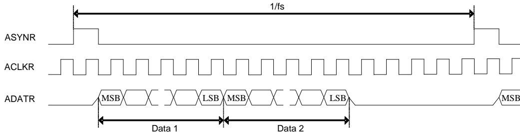
FIGURE 12. ACLKMASTER=0, RM_SYNC=1
