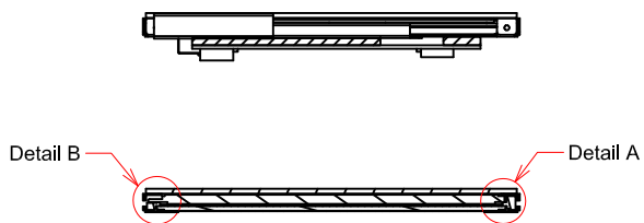
Section H2-H2
